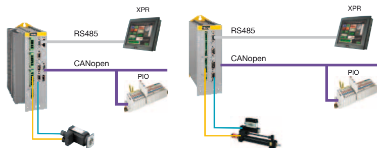
C3S / C3H / C3M I21T30/T40 (CANopen)
